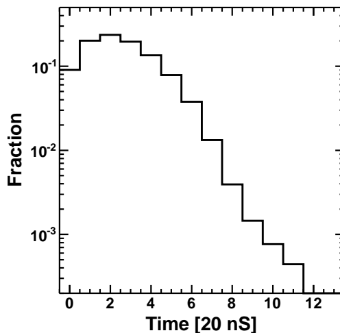
Figure 4.6: Response shape to a minimum ionizing particle for a typical TA SD counter.
