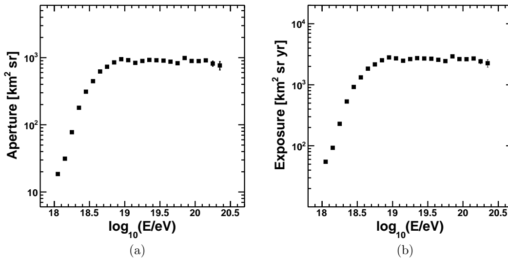
Figure 6.2: Generalized TA SD aperture and exposure calculated by the Monte-Carlo method (Equation 6.10). Small-scale features in these quantities seen at E \sim 10^{19} eV and E \sim 10^{19.8} eV are caused by rapid changes in the detector efficiency and the power law of the (MC) input energy spectrum, respectively. (a): Generalized TA SD aperture. For E > 10^{18.9} eV, the aperture becomes \sim 890 km 2 sr. (b): Generalized TA SD exposure over 1080 days of data. Above 10^{18.9} eV, the exposure is \sim 2640 km 2 sr. Both (generalized) aperture and exposure include the detector efficiency and the effects of the resolution.
