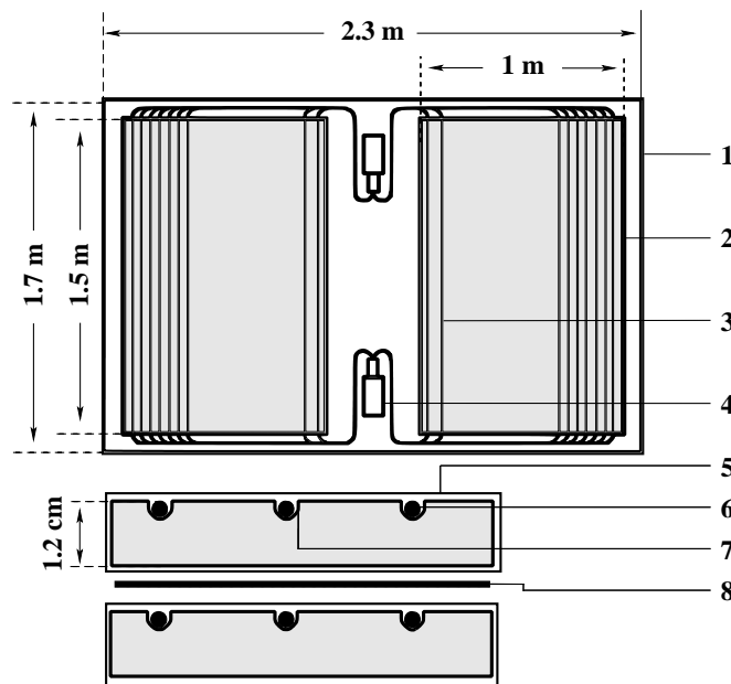
Figure 2.8: TA SD interior configuration, top view (top) and the cross-sectional view (bottom). 1 - Stainless steel enclosure box, 2 - Scintillator (right side of, represented by the shaded area), 3 - Wavelength shifting fiber (WLS), 4 - Photomultiplier tube, 5 - Tyvek sheet, 6 - WLS (cross section), 7 - Grooves for the WLS placement, 8 - Separator plate
