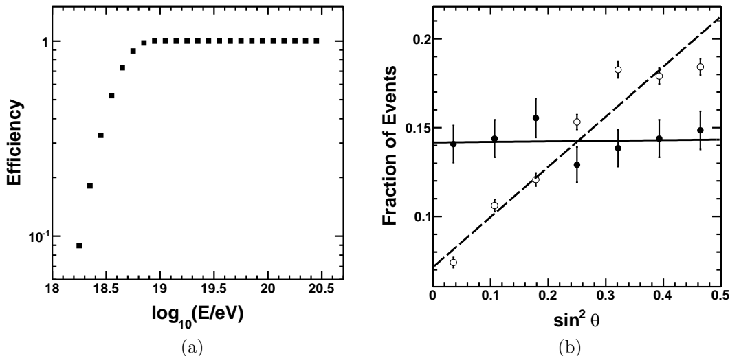
Figure 6.1: (a): TA SD Reconstruction efficiency. 100% efficiency plateau ( E > 10^{18.9} eV) corresponds to the (geometric) aperture value A\Omega = 890 km 2 sr. (b): Normalized distributions of the event \sin^2\theta for E < 10^{18.9} eV (open circles) and E > 10^{18.9} eV (filled circles). Dashed and solid lines show linear fits to these distributions. Above the 10^{18.9} eV threshold, the acceptance does not depend on the zenith angle: the slope of the solid line is 0.003 \pm 0.03 .
