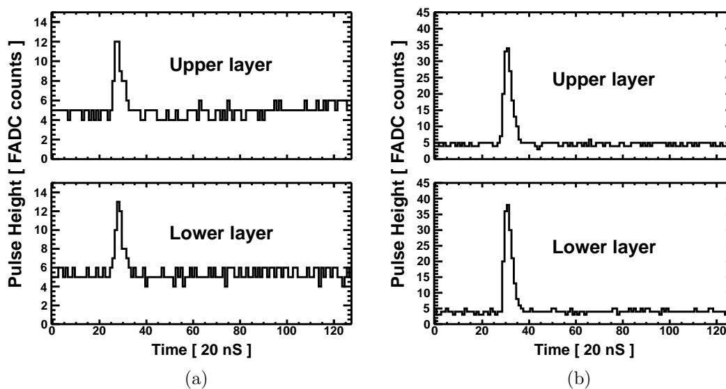
Figure 2.12: TA SD Waveforms: (a) corresponds to the Level-0 and (b) to Level-1 triggers. Flat regions surrounding the pulses, called pedestals , are \sim 5 FADC counts / time slice in these examples.
