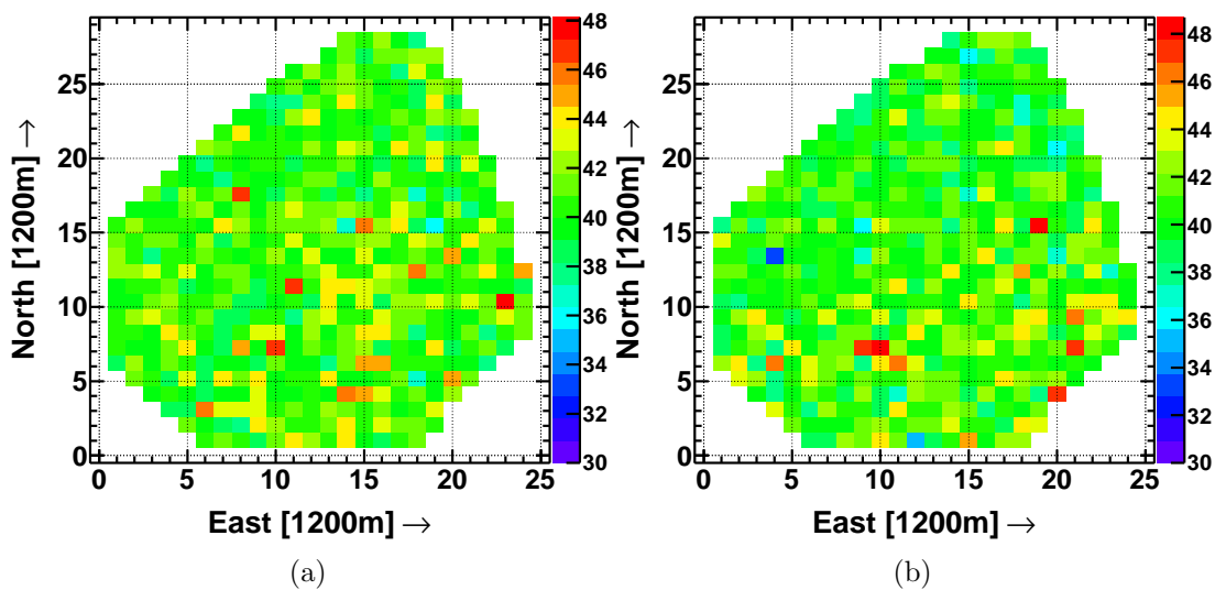
Figure 3.4: Mean gain in FADC counts per VEM, represented by color, over a typical day of data: (a) for the upper scintillator layers, (b) for the lower layers. The gain is plotted versus counter X-Y position.
