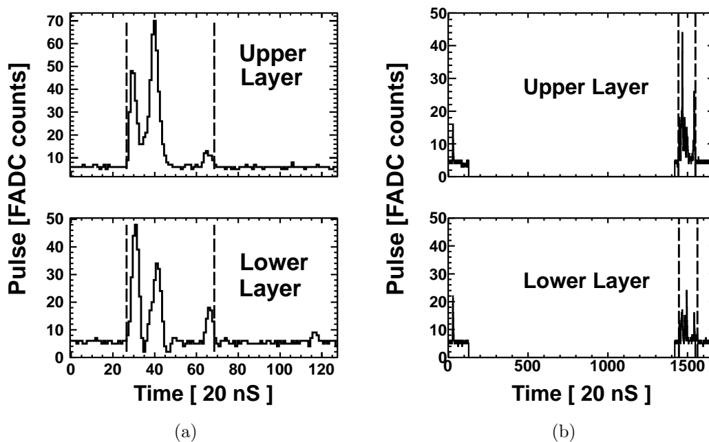
Figure 5.1: Examples of the (processed) counter signals. Dashed lines show the signal selection. In both plots, the left dashed lines indicate the leading edges of the pulses, which define the counter time. (a): An example of a typical signal that is a part of the shower. (b): A signal from the shower (contained within the dashed lines) that was preceded by a random muon pulse, which occurred \sim 25\mu S earlier. Then the counter was silent for \sim 25\mu S (no Level-0 trigger), and finally, the counter triggered again due to the signal from the shower. The random muon pulse was excluded by the signal selection algorithm.
