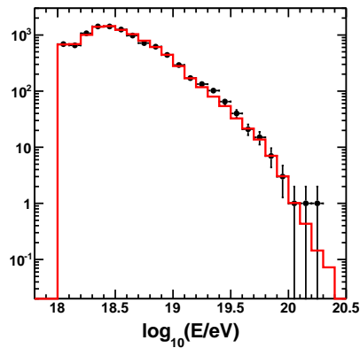
(f) Energy.
