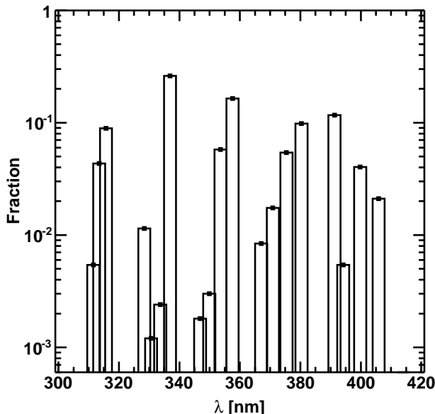
Figure 1.1: Air-fluorescence spectrum measured by the FLASH experiment. Bar widths have been chosen to represent the resolution of the instrument at each point ( \pm 2\text{nm} ).
