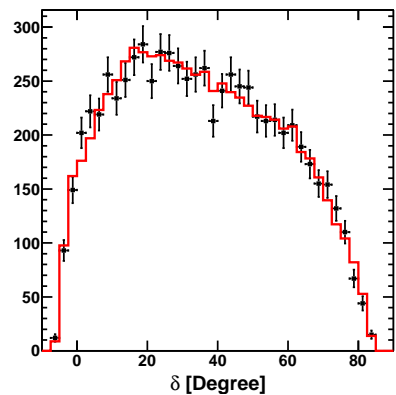
(f) Declination.
