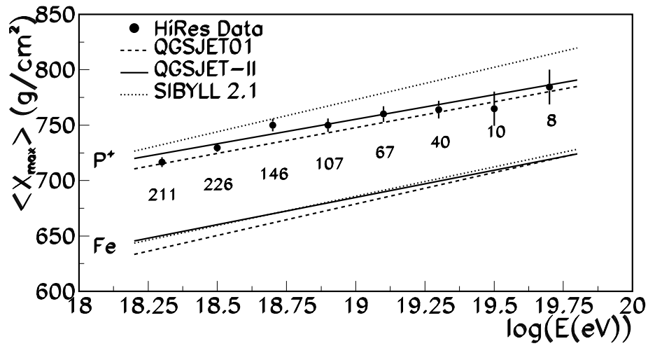
Figure 1.2: HiRes mean x_{\max} result [2]. Points with error bars are the data and lines represent the predictions of the hadronic models for the proton and iron primaries. According to this result, the UHECR primary particles consist of mostly protons above 1.6 \times 10^{18} eV.
