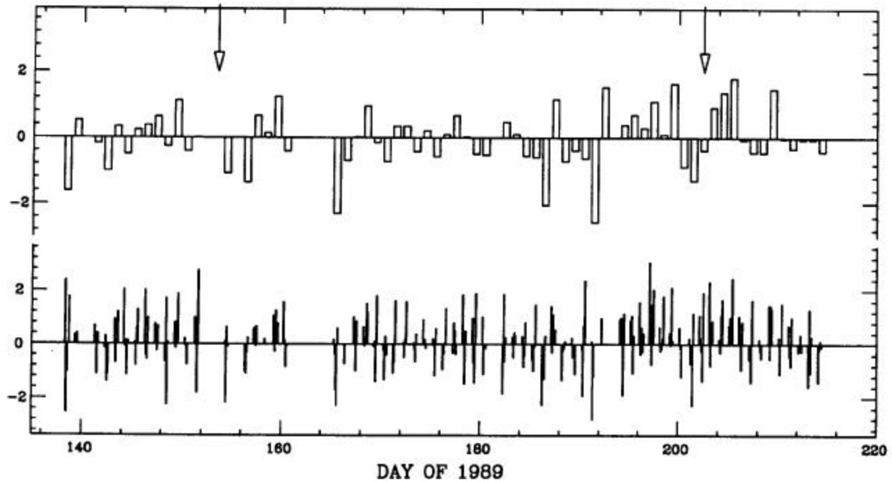
FIG. 1. Significance (Ref. 12), \sigma , of the rate of events from Cygnus X-3 when compared to the expected background measured from off-source data. Upper figure has a bin size of 1 day; lower figure's bins are 2.4 h. Arrows indicate times of peak radio intensity (Ref. 4).
