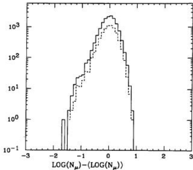
FIG. 2. Distribution of the relative muon content of showers, corrected for zenith angle and N_e . \gamma showers should have less than one-tenth the expected mean number for hadron showers of similar size (i.e., < -1.0 in the figure; see text). Dashed histogram: events from within 3^\circ of Cygnus X-3; solid histogram: combined off-source events from two regions with same declination as Cygnus X-3 but right ascensions offset by \pm 6^\circ . Total off-source solid angle accepted here is twice that of the on-source region.
