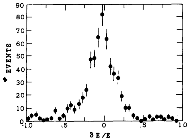
FIG. 3. Monte Carlo response function (E_{in}-E_{out})/E_{in} . Virtually no systematic shift is indicated between Monte Carlo assigned energies E_{in} and analyzed energies E_{out} . Resolution of \pm 15\% is identical with assessed resolution of real data and exhibits almost no energy dependence.
