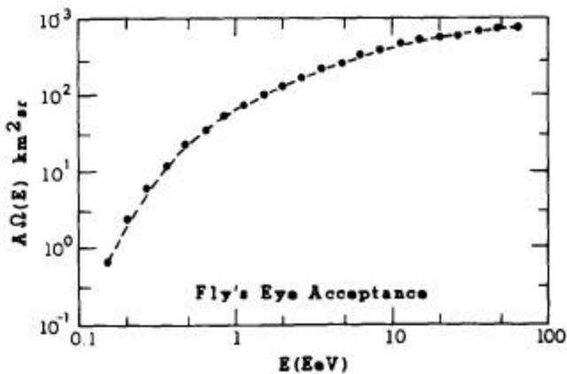
FIG. 1. Fly's Eye acceptance A\hat{U}(E) for events with energy between E and E + dE . Acceptance is based on triggering efficiencies obtained from a Monte Carlo simulation of the Fly's Eye experiment (Ref. 6) and then corrected for track reconstruction and longitudinal development fitting efficiencies.
