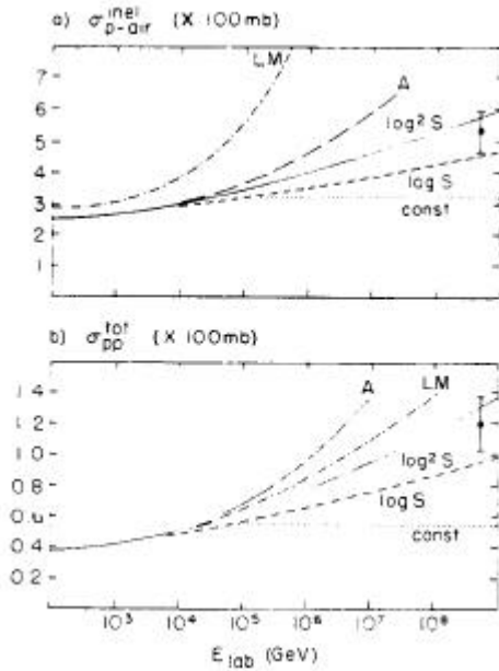
FIG. 6. Energy dependent (a) p-air inelastic and (b) pp total cross sections. The logs and log 2 are extrapolations of fits up to energies of the CERN Intersecting Storage Rings. The curve labeled A is an extrapolation of the estimate of Afek et al. (Ref. 11) and LM stands for Leader and Maor (Ref. 12).
