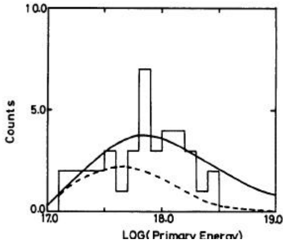
FIG. 3. The energy distribution of observed events from the direction of Cygnus X-3. The dashed line shows the expected background cosmic rays with the present energy-dependent effective area. The solid line shows the combined spectrum obtained by adding a spectrum with an exponent of -1.1, normalized to the observed excess events between 10^{17} and 3 \times 10^{18} eV, to the expected background.
