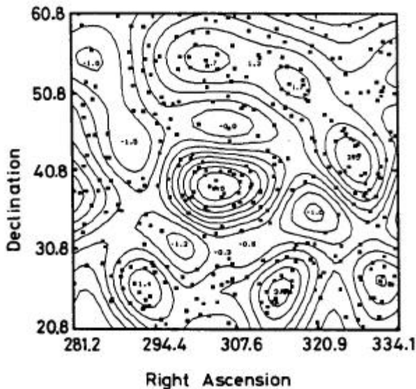
FIG. 1. The significance of the density excess at energies above 5 \times 10^{17} centered on Cygnus X-3 (Akeno 20-km 2 array data) shown by contour lines of 0.5 steps with the arrival direction of each event.
