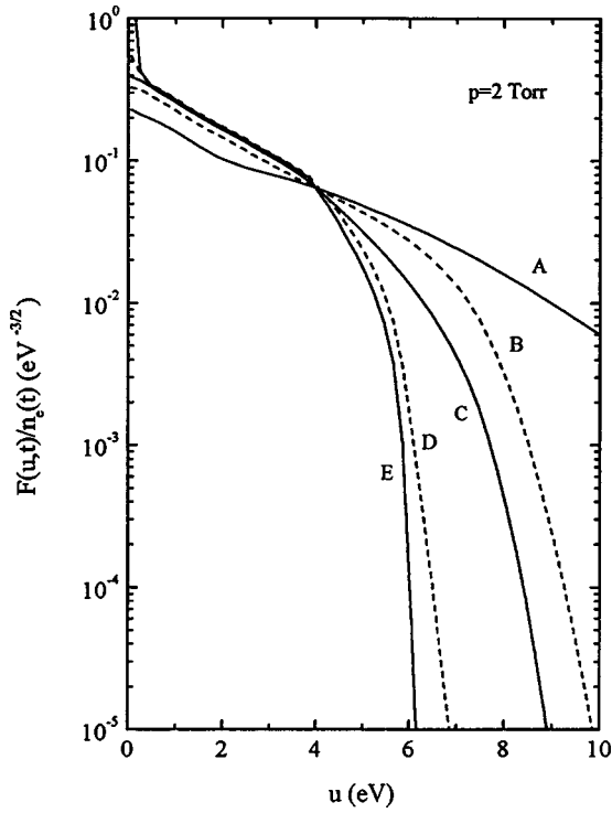
FIG. 1. EEDF calculated in the post-discharge of an \omega/(2\pi) = 2.45 GHz microwave discharge in N_2 , with p=2 Torr and n_e(0)=5 \times 10^{11} \text{ cm}^{-3} , for the following instants in the afterglow: (A) t=0 , (B) 10^{-7} s, (C) 10^{-5} s, (D) 10^{-4} s, (E) 3.2 \times 10^{-4} s.
