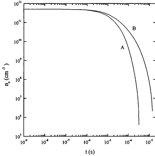
FIG. 12. Temporal evolution of the electron number density in the post-discharge of an \omega/(2\pi) = 2.45 GHz microwave discharge in N_2 , with n_e(0) = 5 \times 10^{11} \text{ cm}^{-3} , R = 0.8 \text{ cm} , and p = 2 Torr (A) and 10 Torr (B).
