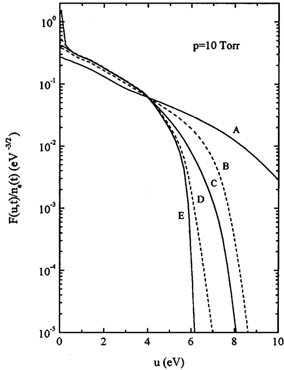
FIG. 15. EEDF calculated in the post-discharge of an \omega/(2\pi) = 2.45 GHz microwave discharge in N_2 , with p=10 Torr and n_e(0)=5 \times 10^{11} \text{ cm}^{-3} , for the following instants in the afterglow: (A) t=0 , (B) 10^{-7} s, (C) 10^{-5} s, (D) 10^{-4} s, and (E) 1.4 \times 10^{-3} s.
