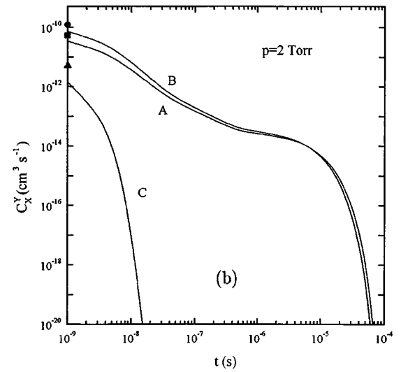
FIG. 5. Temporal evolution of the electron rate coefficients for excitation of N_2(A) , N_2(B) , and N_2(C) states [curves A–C in Fig. 5(a)], and for excitation of N_2(a') and N_2(a) states plus ionization [curves A–C in Fig. 5(b)], calculated in a N_2 afterglow for the same conditions as in Fig. 1, using our reference model for electron diffusion and including e - e collisions. The symbols represent the rate coefficients in the discharge ( t=0 ).
