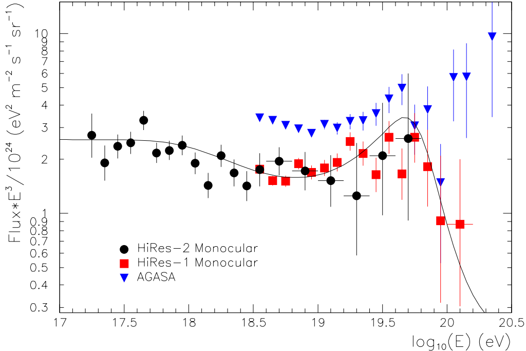
Fig. 1. The two HiRes monocular spectra, along with the AGASA spectra. A fit to the HiRes spectra to a two component model is also shown
