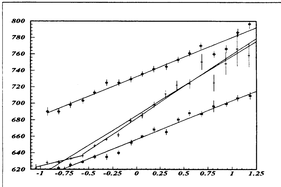
Figure 1: Elongation rate, data ( crosses ), Fe ( stars ) and protons ( circles ). X axis is \log_{10}(E) . Y axis is X_{\max} in \text{gm}/\text{cm}^2 . The error bars indicate the statistical error on the mean.
