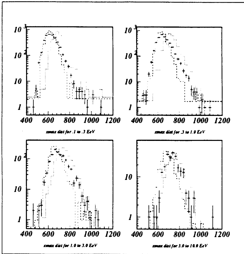
Figure 2: X_{\max} distribution for data (crosses), Fe (short dashes) and protons (long dashes) for four energy bins: 0.1 to 0.3 EeV .3 to 1.0 EeV; 1.0 to 3.0 EeV; and 3.0 to 10.0 EeV.
