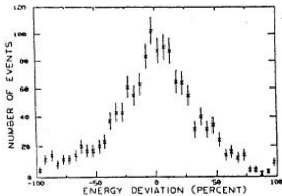
Figure 2. % Differences Between Measured Shower Energy and Known Monte-Carlo Input Energy.
