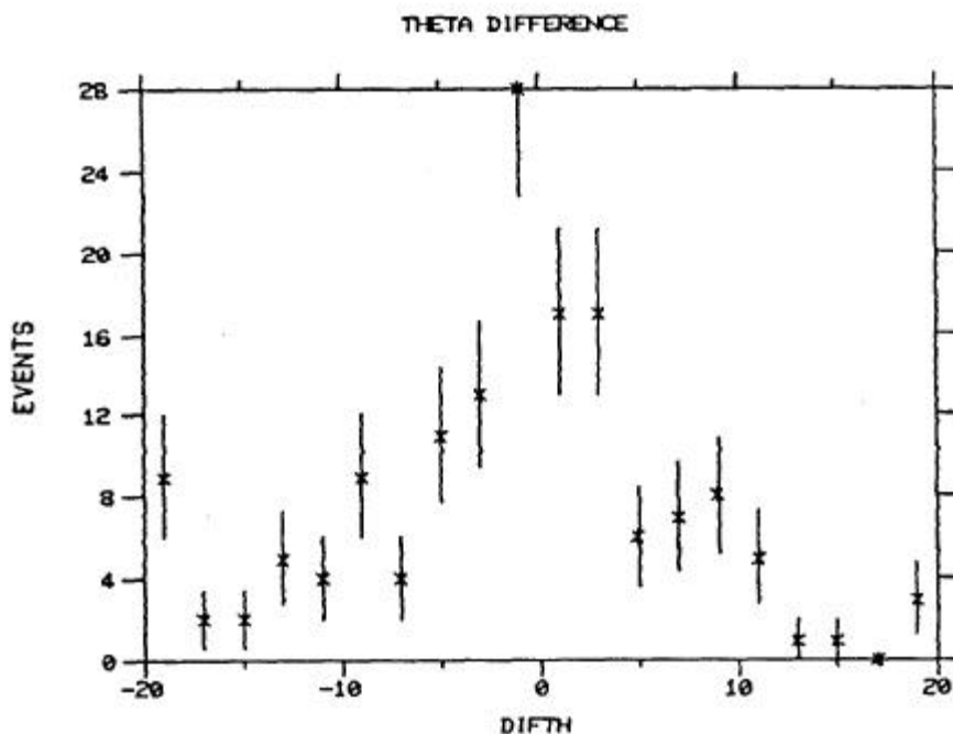
Figure 3. Difference in Zenith Angle for Events Observed by Both Detectors and With One Detector Alone. The average angular length for the track is about 40°.
