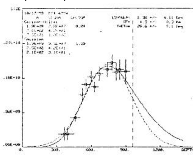
Figure 1. An Extensive Air Shower at Survives All Data Cuts. The solid curve is a GH. shower curve. The dotted curve is a Gaussian distribution.
