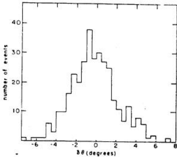
Figure 2. Distribution of differences between known and fitted zenith angles for "upward-going" showers of known geometry generated by a high intensity light flasher. The width of the distribution is \sigma = 1.7^\circ .
