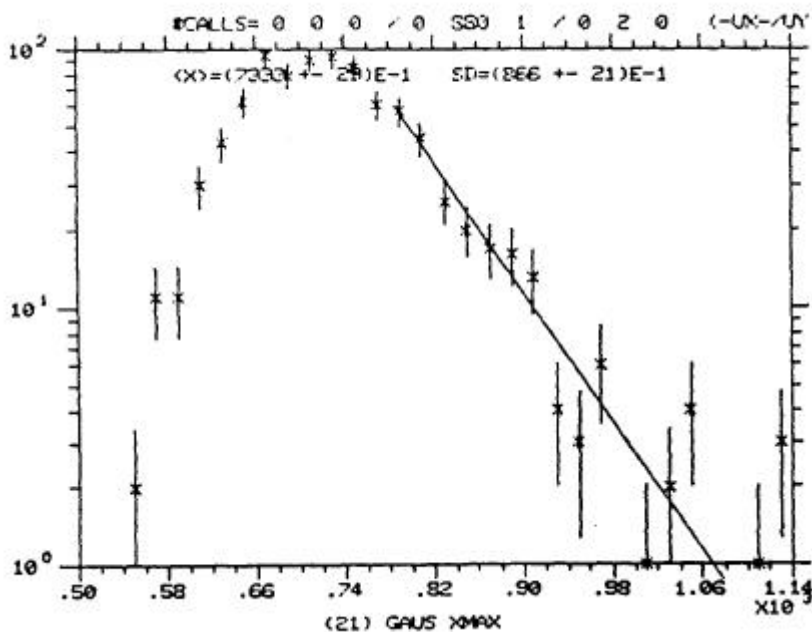
Figure 4. Distribution of Depth of Shower Maxima for Data Whose Fitting Errors Are Less Than \pm 100 \text{ g cm}^{-2} . The slope of the exponential tail is \lambda = 70 \pm 6.9 \text{ cm}^{-2} .
