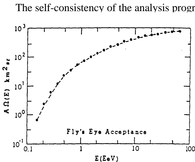
Figure 3. Fly's Eye Sensitive Aperture.
