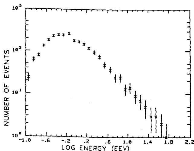
Figure 1. Raw Energy Distribution of Fly's Eye Data.
