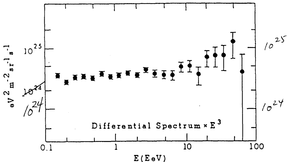
Figure 5. Fly's Eye Differential Energy Spectrum.
