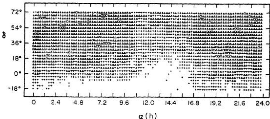
Figure 1. Flux upper limits at the 95% confidence level are represented by the following symbols: squares ( F < 3 \times 10^{-13} \text{ cm}^{-2} \text{ s}^{-1} ), triangles ( 3 \times 10^{-13} < F < 10^{-12} \text{ cm}^{-2} \text{ s}^{-1} ), and plus signs ( 10^{-12} < F < 3 \times 10^{-12} \text{ cm}^{-2} \text{ s}^{-1} ).
