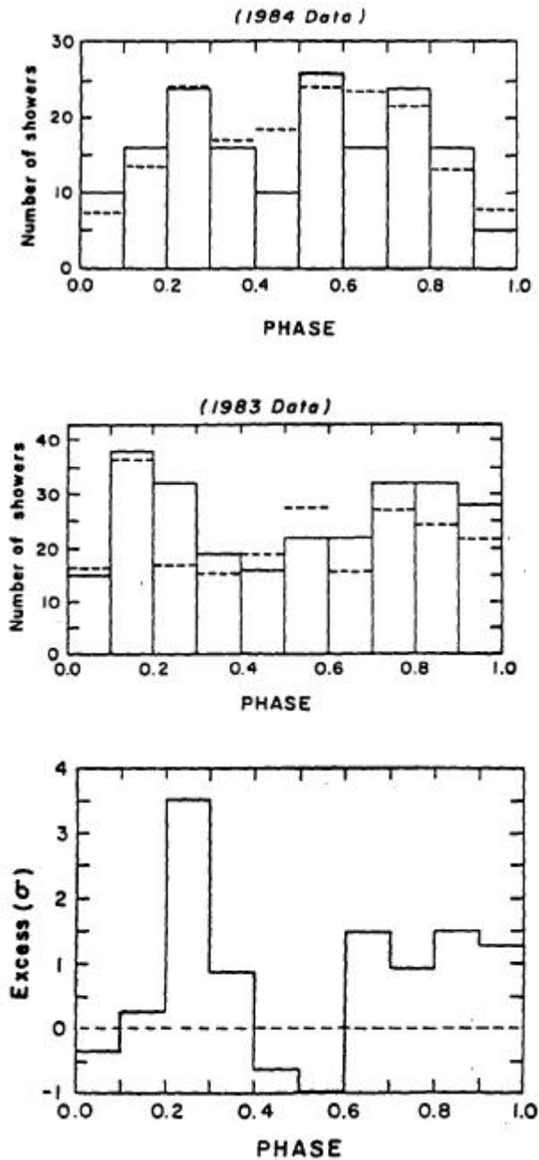
Figure 2. Parts a and b show the light curves within the 4.8h Cygnus X-3 period for (a) the 1984 data, and (b) the 1983 data. Expected background levels are shown by the dashed lines. In part c, the statistical significance of deviations are plotted for the 1983 data..
