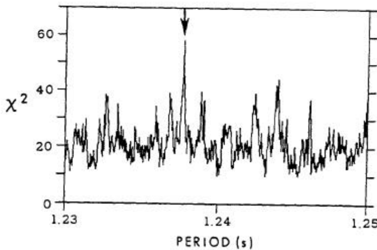
Fig. 2 The \div 2 dependence on the period used to ford the data. The arrow marks the period obtained from Nagase et al. 1984.
