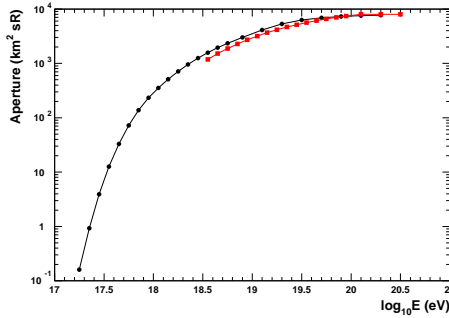
Fig. 6. The calculated apertures of HiRes-I (red squares) and HiRes-II (black circles) as a function of energy, using the average X_{\max} measurements from HiRes/MIA [20] and HiRes Stereo [21].
