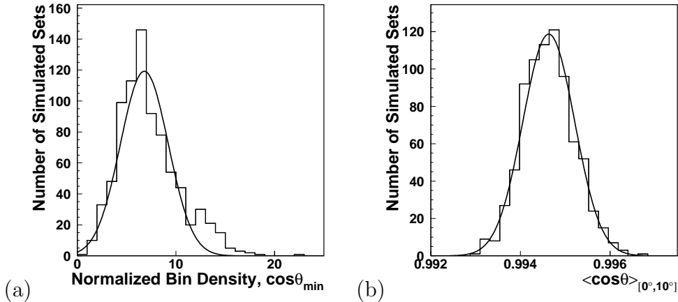
Fig. 7. Distributions of normalized bin densities of \cos\theta_{\min} and \langle \cos\theta \rangle_{[0^\circ, 10^\circ]} values for a large number of simulated sets with the same level of clustering as in figure 6—(a) Distribution of observed normalized bin densities of \cos\theta_{\min} , note that it is not Gaussian ( \chi^2/dof = 5.44 ); (b) : \langle \cos\theta \rangle_{[0^\circ, 10^\circ]} distribution ( \chi^2/dof = 1.09 ).
