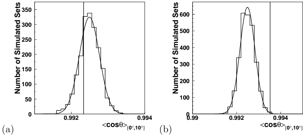
Fig. 12. Distribution of \langle \cos \theta \rangle_{[0^\circ, 10^\circ]} values for simulated isotropic data sets—(a) HiRes-I; (b) AGASA. In each figure, the vertical line represents the the value of \langle \cos \theta \rangle_{[0^\circ, 10^\circ]} for the observed data.
