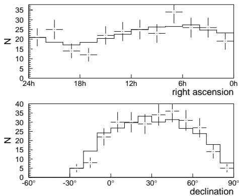
FIG. 2.— Right ascension and declination of events above 10^{19} eV observed from 1999 December through 2004 January. (Data—points with error bars; Monte Carlo—solid line.) For right ascension, \chi^2/\text{dof} = 0.77 ; for declination, \chi^2/\text{dof} = 0.73 .
