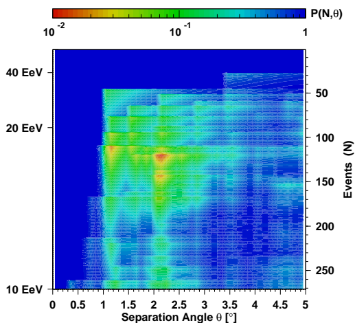
FIG. 3.— Autocorrelation scan of the HiRes data set above 10^{19} eV. P(N, \theta) is the probability of obtaining the same or greater number of pairs as is actually observed in the data using a maximum separation angle \theta and searching among the N highest-energy events. These probabilities do not include the statistical penalty due to scanning.
