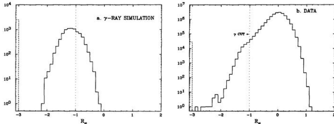
FIG. 4.-Distribution of the relative muon size R_\mu , (eq. [4]) for (a) simulated \gamma -ray showers and (b) data. Eighty percent of simulated \gamma -ray events have R_\mu < -1.0 , shown by the dotted line. Data with R_\mu < -1.0 (i.e., to the left of the dotted line) are retained as candidate \gamma -ray showers. In each figure, showers with no recorded muons are plotted as underflows in the dashed bin at the left
