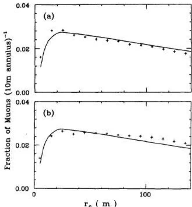
FIG. 3.-Lateral distributions of muons as measured by accumulated hits in the buried counters (a) for showers within 5^\circ of the zenith and (b) for showers slanting at more than 30^\circ to the zenith. The points represent the fraction of the total number of buried counter hits accumulated in annular rings of width 10 m and distances r , from the shower axis. Error bars are slightly less than the size of the plot symbols. The solid curves are calculated from the lateral distribution function of Greisen (eq. [2]) with a 10 m smearing of the function to account for errors in measuring positions of shower cores. The distributions contain showers with N > 3 \times 10^4 . Punch-through is evident as an excess of hits close to the core. The amount of punch-through decreases at large zenith angles due to increased absorption in air and earth.
