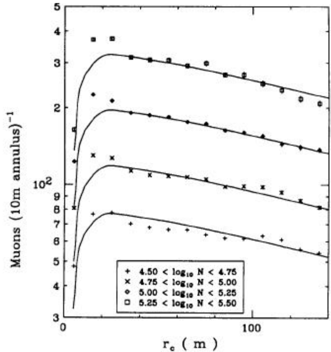
FIG. 2.-Lateral distributions of moons for cosmic ray showers within 5^\circ of vertical. The different groups of data refer to showers with different sizes as measured by the counters on the surface. The points represent the average number of hits in the buried counters, accumulated in annular rings of width 10 m and distances r , from the shower axis. The solid curves are calculated from the lateral distribution function of Greisen (eq. [2]) with a 10 m smearing of the function to account for errors in measuring positions of shower cores. Punch-through is evident as an excess of hits close to the core. The amount of punch-through increases with shower size.
