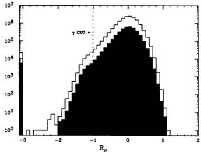
FIG. 5.-Distribution of relative muon size R , (eq. [4]) as in Fig. 4b, except here the data are divided into two groups: Galactic ( shaded area ) and non-Galactic events. Showers with no recorded muons are plotted as underflows in the leftmost bin. Events with R_i < -1.0 (i.e., to the left of the dotted line) are retained as candidate \gamma -ray showers.
