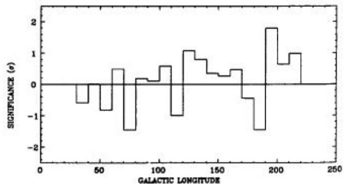
FIG. 6.-Significance of observed number of muon-poor showers with respect to the expected number along the Galactic plane ( |b^{\text{II}}| < 10^\circ ). The bin size is l^{\text{II}} = 10^\circ . The significance is expressed in units of Gaussian standard deviation \sigma , calculated as in Li & Ma (1983).
