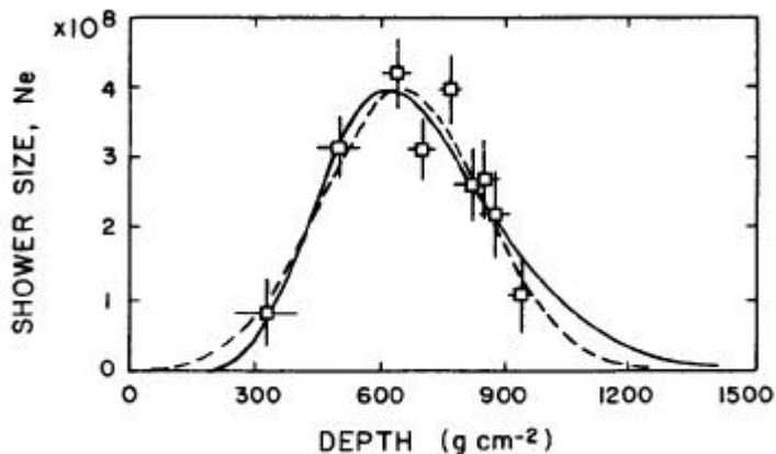
FIG. 1.-A typical shower development profile as measured by the stereo Fly's Eyes. Two fits to the data are shown, Gaussian ( dashed line ) and GaisserHillas ( solid line ). Results from the Gaussian fit given an energy of (4.6 \pm 0.4) \times 10^{17} eV and a depth of maximum of 650 \pm 39 g cm -2 .
