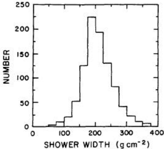
FIG. 6.-The distribution of shower widths for showers with energies larger than 3 \times 10^{17} eV, estimated relative X_{max} error less than 0.12 and all viewing angles larger than 20^\circ . The parameter plotted is the standard deviation of the Gaussian shower profile function. The mean value of the distribution is 207 \pm 2 g cm ^{-2} with a width (standard deviation) of 50 \pm 1 g cm ^{-2} .
