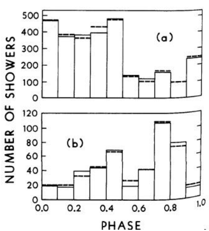
FIG. 4.-Data from 1985 October 17 18, and 19, following the Cyg X-3 radio outburst. Observed (solid lines) and expected (dashed lines) numbers in good agreement for (a) all E and (b) E > 100 TeV. Flux limits are given the text.
