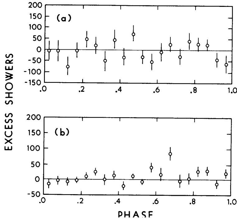
FIG. 3.-Combined data from 1985 June, July, and August. Observed minus expected numbers are given as a function of the 4.8 hr phase. (a) E = 10-100 TeV ; (b) E = 100-1000 TeV. The upper E interval shows an excess in phase 0.65-0.70.
