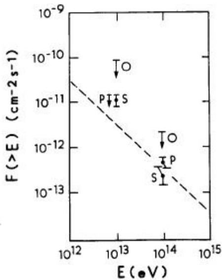
FIG. 5.—Observed flux values and flux upper limits are given for the 1985 October run (O), periodic signals in 1985 summer (P), and the 1955 June 17 sporadic effect, averaged over the total summer observing time (S). The dashed line is a comparison spectrum from Lloyd-Evans et al. (19836).
