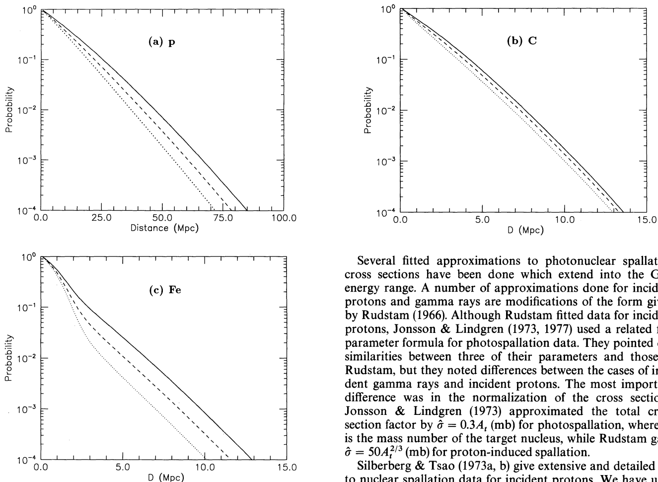
FIG. 3.—Probability of sources at various distances, considering only propagation effects (see discussion in text). Spectra with differential spectral indices of 2, 2.5, and 3, are indicated by solid, dashed, and dotted curves, respectively. Results are given for (a) protons, (b) carbon nuclei, and (c) iron nuclei.
