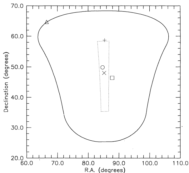
FIG. 4.—The source search region is shown by the outer boundary. It is defined by angular distances of 10^\circ from the 2 \sigma error box shown by the dotted lines. The best-fit shower direction is shown by the cross. The circle and square represent the directions of 3C 147 and MCG 8-11-11, respectively. The triangle shows the direction of NGC 1569 (also known as Arp 210.) The + symbol is in the direction of UGC 03351, also known as MCG10-09-02. See text for details.
