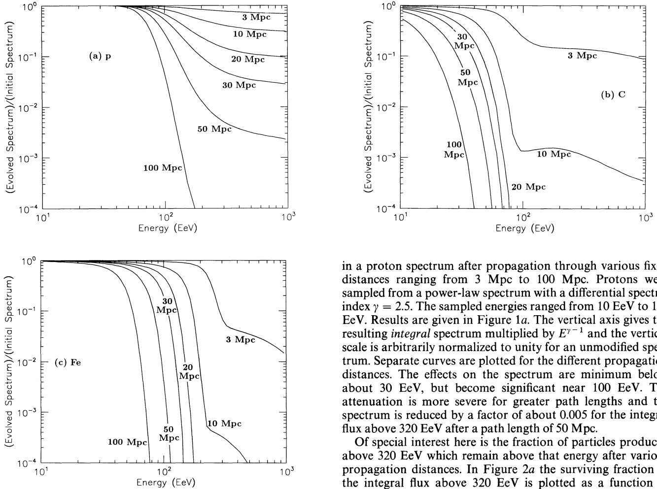
FIG. 1.—Integral flux reduction factors as a function of energy, after a spectrum with a differential spectral index of 2.5 has been propagated the indicated distances. Results are given for the following initial particles: (a) protons, (b) carbon nuclei, and (c) iron nuclei.
