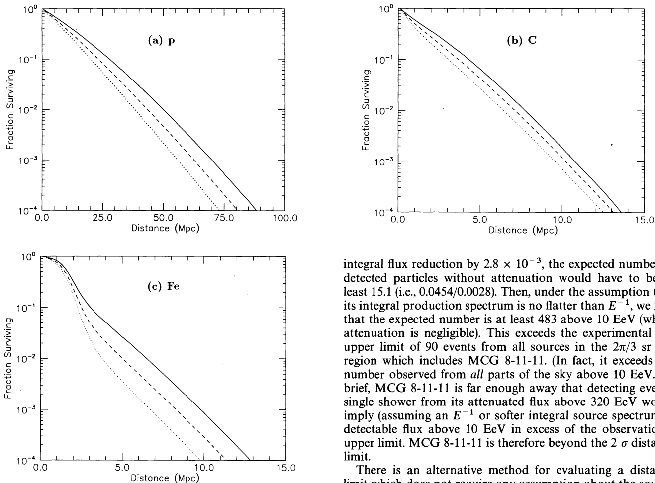
FIG. 2.—The dependence of the integral flux reduction factor on path length for cosmic rays with energies greater than 320 EeV. Spectra with differential spectral indices of 2, 2.5, and 3, are indicated by solid dashed, and dotted curves, respectively. Results are given for (a) protons, (b) carbon nuclei, and (c) iron nuclei.
