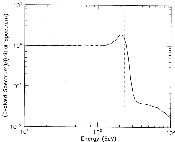
FIG. 5.—Ratio of surviving differential flux to source flux for primary iron nuclei as a function of the detected energy after a path length of 3.5 Mpc. The differential spectral index was chosen to be \gamma = 2.5 . A “pile-up” is observed near the shower energy (230 EeV, marked by a dotted line) proposed in a scenario involving acceleration of the cosmic ray near M82. (See text.)
