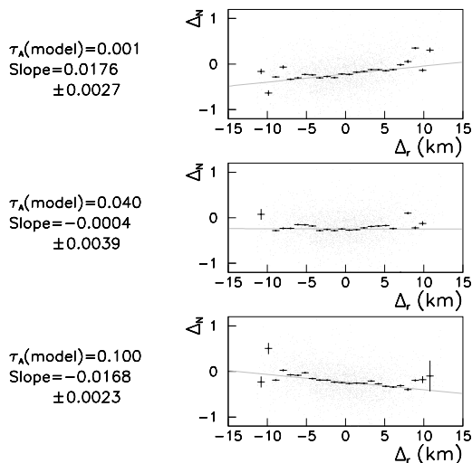
Fig. 3.— Plots of \Delta_N (light balance) versus \Delta_r (path difference) for real data using three different model atmospheres ( \tau = 0.001, 0.040, \text{ and } 0.100 ). The model with \tau = 0.040 results in the smallest slope.
