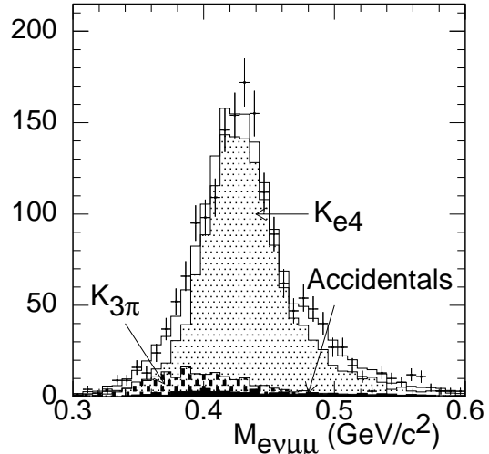
FIG. 5: Projection onto the m_{e \nu \mu \mu} axis of the data of Fig. 3 (points) and of the fitted distribution (unshaded histogram). The three background contributions are shown separately (shaded histograms).
