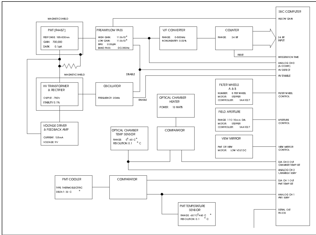
Figure 1-3. Circuit function diagram.
