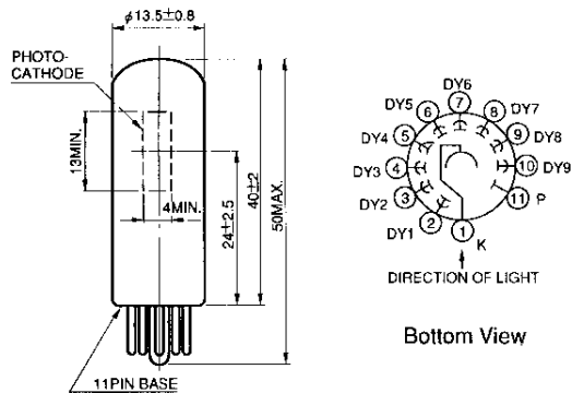
Figure 3: Dimensional Outline and Basing Diagram (Unit:mm)
