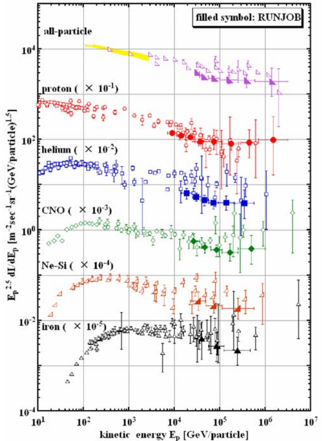
Figure 4. Final hydrogen - iron spectra obtained by RUNJOB (solid points) compared to other measurements and the all-particle spectrum [6]. In particular, note that the absolute proton intensities reported by RUNJOB (●) and JACEE (○) are in reasonable agreement while the helium intensities (■ and □ respectively) differ by approximately a factor of 2.
