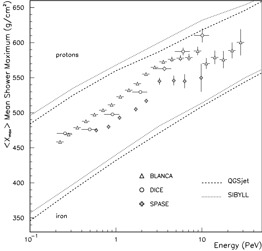
Fig. 3. Results from experiments reporting \langle X_{max} \rangle [39,37,53]. Also shown are the results from model calculations discussed in text. The SIBYLL [41] calculation is from Table 1, the QGSjet is from [42].
