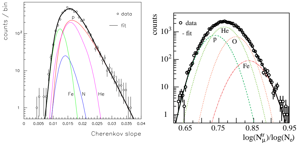
Fig. 12. Two examples of multi-species fits to air shower observables; BLANCA[39] at left, KASCADE[80] at right. See text for details.
