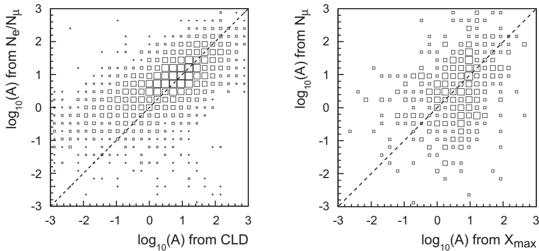
Fig. 13. Two examples of event-by-event correlations between mass estimates near 3 PeV derived from different air shower observables; BLANCA[39] at left from Cherenkov Lateral Distribution and Electron Muon sizes, DICE[37] at right from the Cherenkov image and Muon sizes. See text for details.
