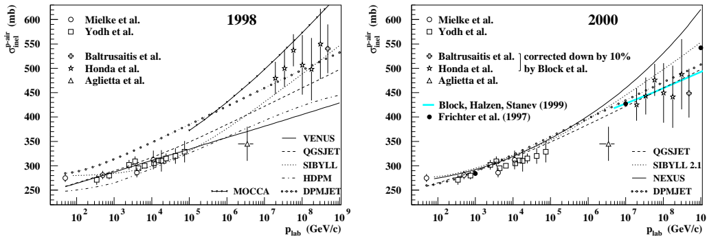
Fig. 4. Inelastic p-air cross-sections. left : Situation in 1998 right : Situation in 2000 data. They simultaneously fit the total p-p cross-sections, the ratio of real to imaginary part of the forward scattering amplitude \rho , and the nuclear slope parameter B . Then the p-p cross-sections were converted via Glauber theory into p-air cross-sections. Their result agrees very well with the cross-sections used in the QGSjet model.
