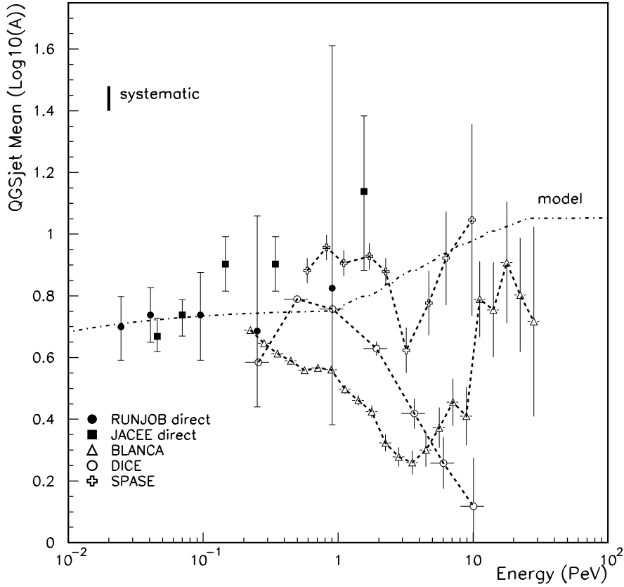
Fig. 9. Results on shower maximum analyzed with the QGSjet model in Figure 3.
