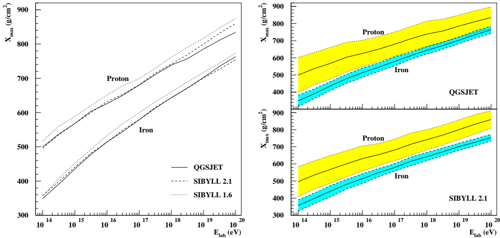
Fig. 6. Height of shower maximum X_{\max} as a function of energy. left : The curves for QGSjet, a preliminary version of SIBYLL 2.1 and SIBYLL 1.6 are shown. right : Average values together with the 1\text{-}\sigma band indicating the standard deviation of the X_{\max} distribution. [76]
