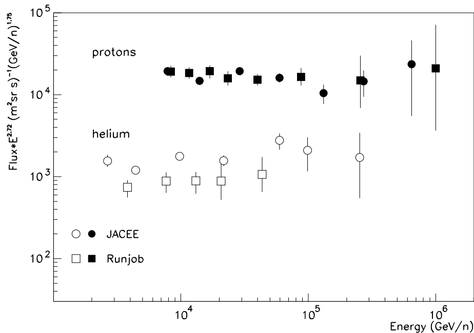
Fig. 2. Direct measurements of cosmic ray components by the JACEE [13] and RUNJOB [15] experiments
